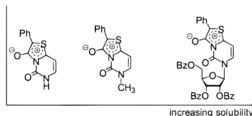
Figure 3. Substituent dependency of the solubility.
