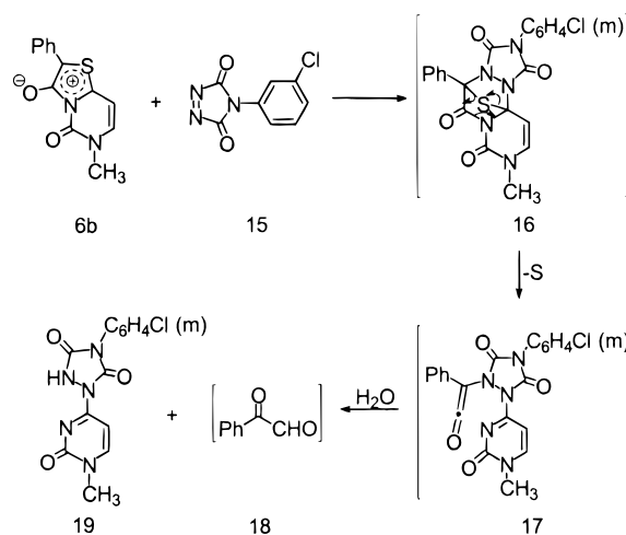
Scheme 4. Suggested Cycloaddition Extrusion Mechanism
